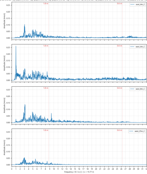
Train 2023111154144762 @ 27.0 m/s | track = 1 | sensor = Schalkwijk_Z | loading = 0% | vehicle.repetition = 8% vehicle types: El Lok 1600/1700/1800 -{2x}(Unknown Vehicle) -{2x}(WAG FACCS/TAGNPPS(1) -{2x}(Unknown Vehicle) -{2x}(WAG ZACENIS(3)-Unknown Vehicle-WAG FACCS/TAGNPPS(1)-WAG ZACENIS(3)-WAG FACCS/TAGNPPS(1)-{3x}(WAG ZACENIS(3))-WAG FACCS/TAGNPPS(1)-Unknown Vehicle-WAG FACCS/TAGNPPS(1)-WAG ZACENIS(3)-{2x}(Unknown Vehicle) axle distance: [2.8-6.9-2.8]-{1.8-8.3-1.8} -{5x}[3.3]-{1.8-9.6-1.8} -{2x}[3.2]-{1.8-8.2-1.8}]-{3x}[3.1]-{1.8-9.6-1.8} -3.2-[1.8-8.2-1.8]-{3x}[3.5]-{1.8-9.6-1.8} -3.5-[1.8-8.1-1.8] -{2x}[3.2]-{1.8-8.2-1.8} -3.2-[1.8-9.6-1.8] -{2x}[3.3]-{1.8-8.3-1.8}
