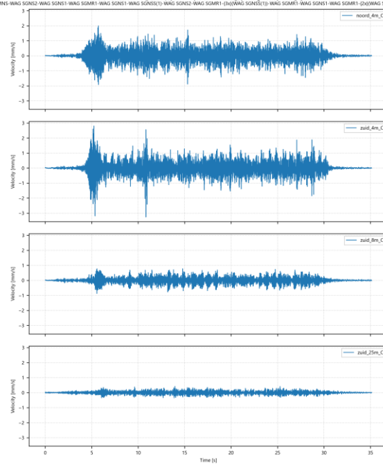
Train 2024020923347775 @ 25.5 m/s | track = 1 | sensor = America Z | loading = 86% | vehicle_repetition = 6% vehicle types: EL BR186 (1x) - (2x)WAG SDOGMN1 - WAG SDOGMRRS - WAG SHIMMNS - WAG SGN52 - WAG SGN51 - WAG SGMRI - WAG SGN51 - WAG SGN51 - WAG SGN52 - WAG SGMRI - (1x)WAG SGN51 - WAG SGMRI - WAG SGN51 - WAG SGMRI - (2x)WAG SGN51 - (3x)WAG SGN51 - WAG SGN51 - (2x)WAG SGN51 - (2x)WAG SGN51 - WAG SDOGMRRS
